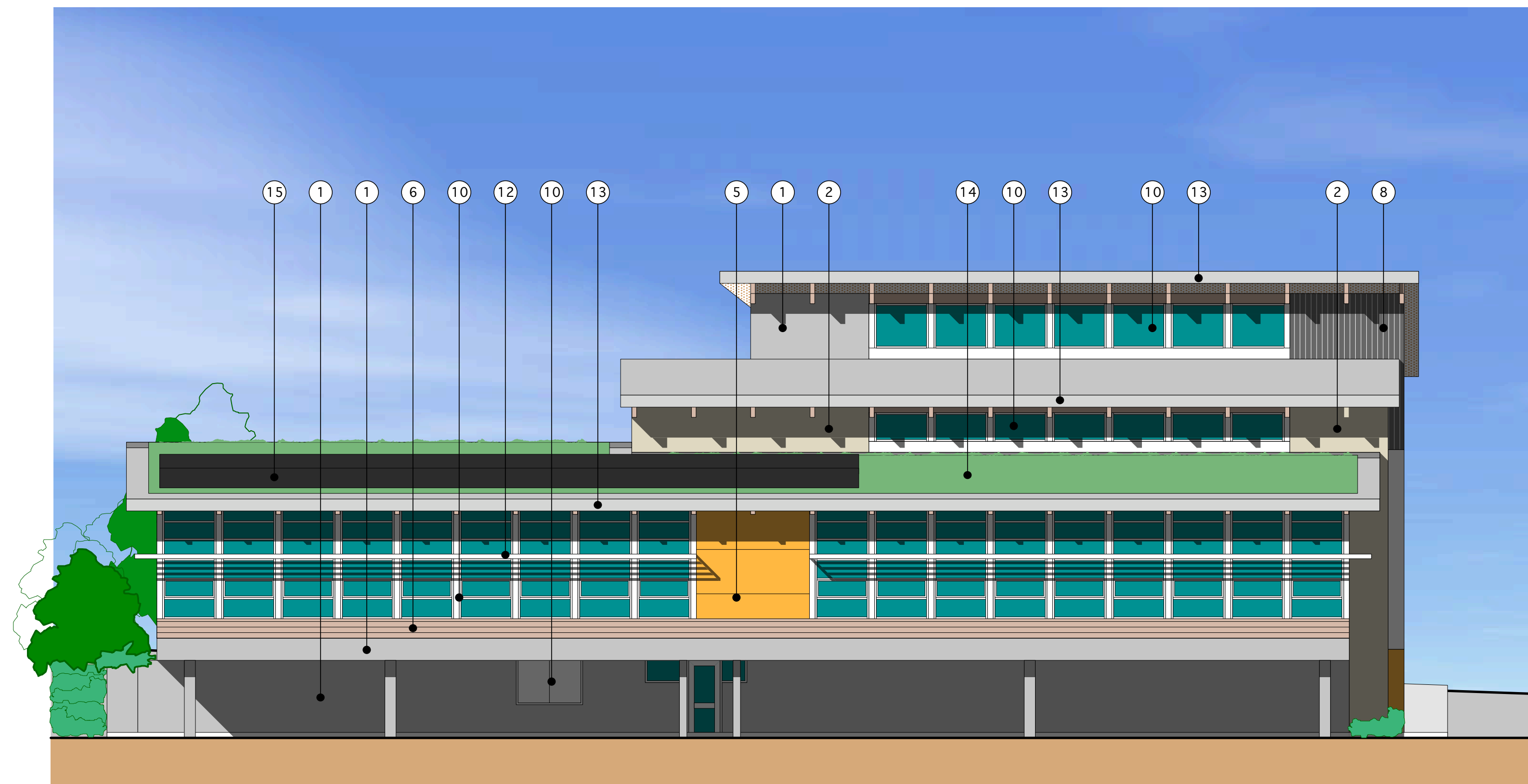
South Elevation
